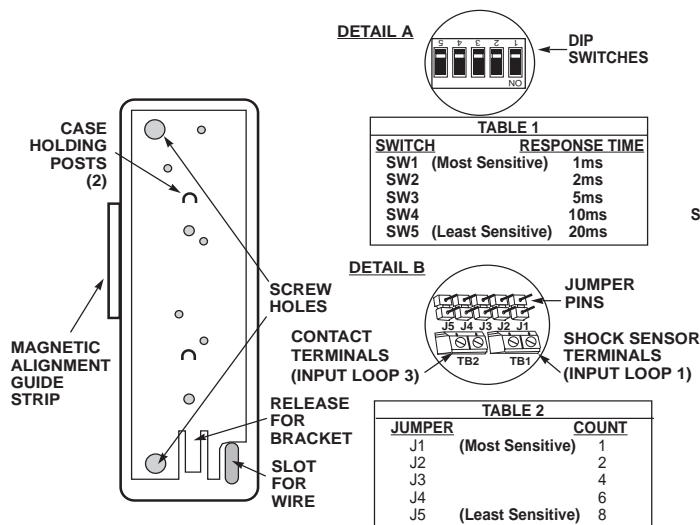
Diagram 1: MOUNTING PLATE
