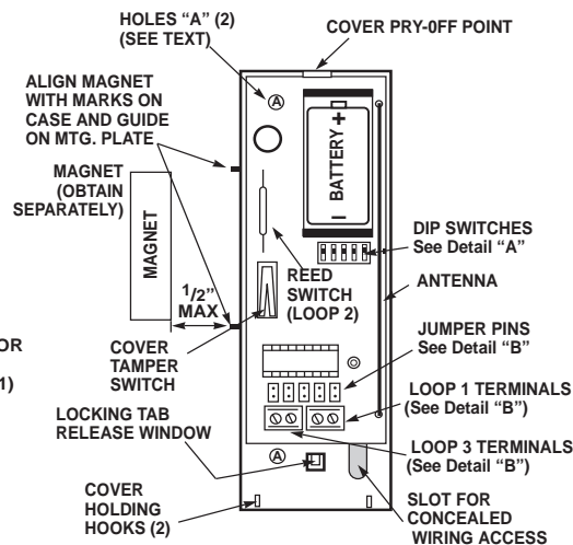
Diagram 2: No. 5819 (SHOWN WITH COVER REMOVED)
